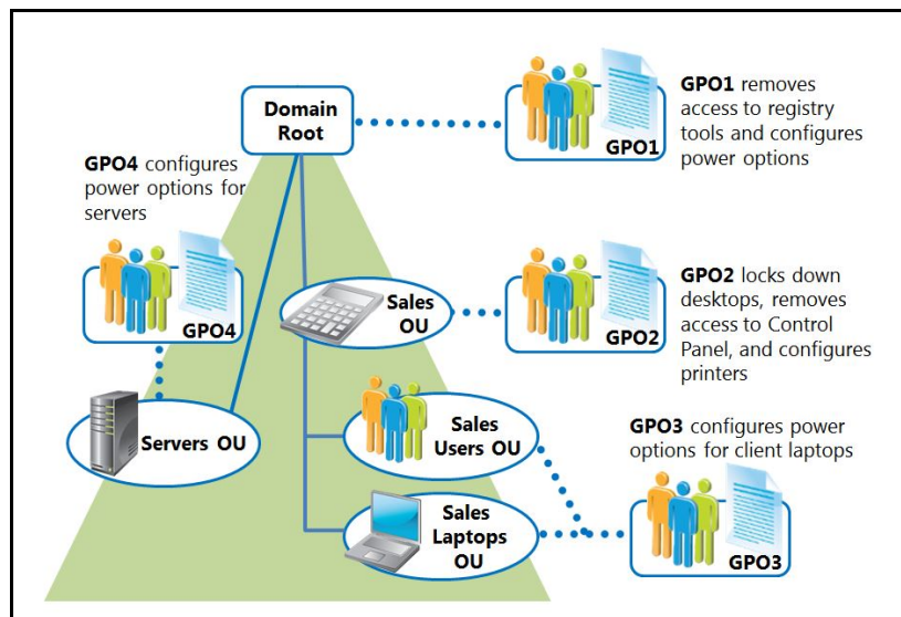
FIGURE 11.1: AD DS STRUCTURE
